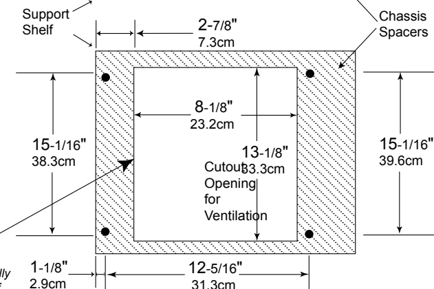
C1100C Bottom View in Custom Cabinet
